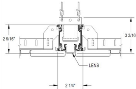
LED Lamping
