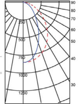
Quadralaterally Symmetric Dashed: 0 Degrees Solid: 90 Degrees
